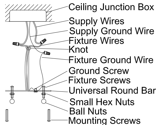
Wiring Drawing ( 2 )
