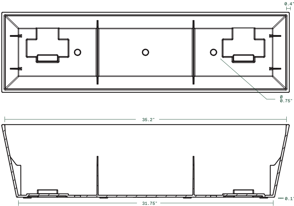
Interior Dimensions
