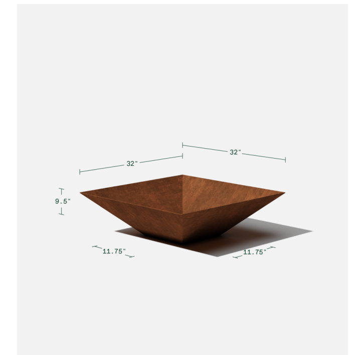
Exterior Dimensions
