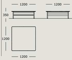
Low console table
