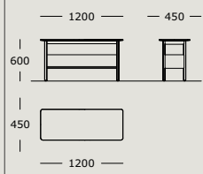
Low console table
