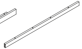
D. Top Back Rail x1 Part# 25106
