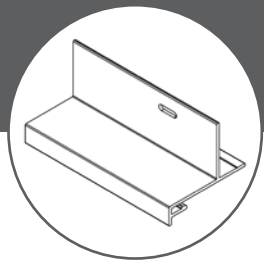
Nailing Fin / Flashing (Snaps into accessory groove) Recommended For New Construction Applications
