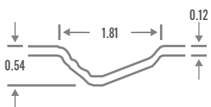
6-PANEL TEXTURED PROFILE
