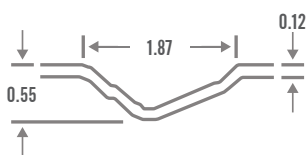
2-PANEL SQUARE & ROMAN, 4-PANEL & 6-PANEL SMOOTH PROFILE
