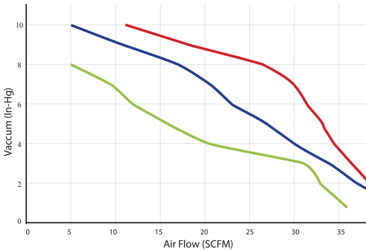
Air Flow vs Vacuum
