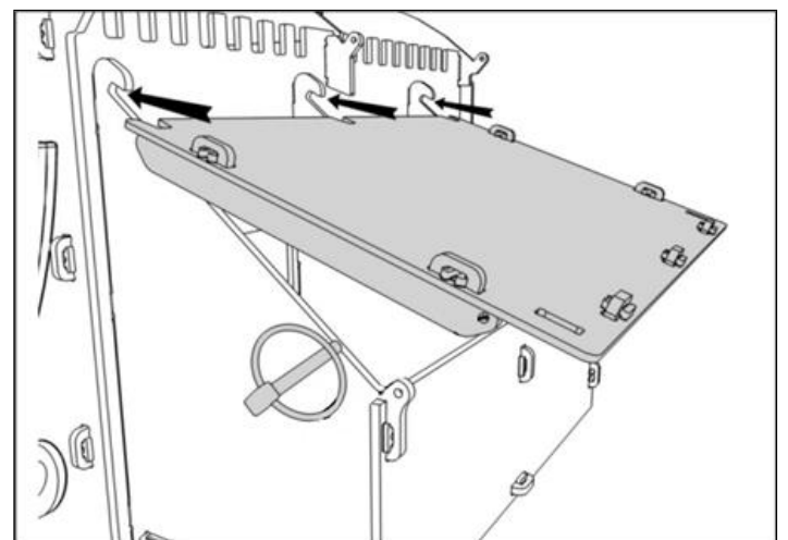
18, The Nest Box Lid simply slides upwards so that the cutouts fit into the recesses in the vertical panels. It is secured with 2x Linch Pins.
