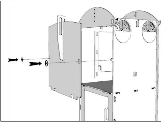
11 Fit the Back Door using 2x Linch Pins. (When fitting, first rest the bottom of the Back Door in the slots in the Base, then push the door onto the lugs, and slide the Back Door Handles downwards. Secure it with Linch Pins.
