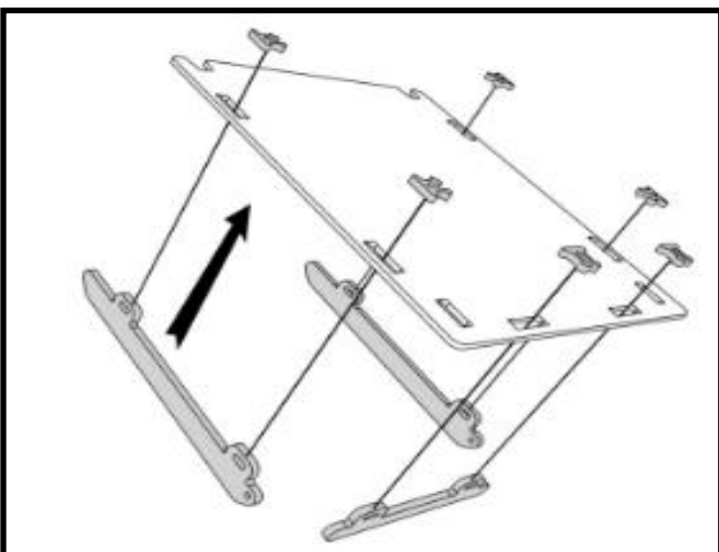
15 Fit the Nest box Front Brace and the two Nest box Side Braces to the Nest box Lid, which should have its patterned side upwards, using 6 x Pi Clips
