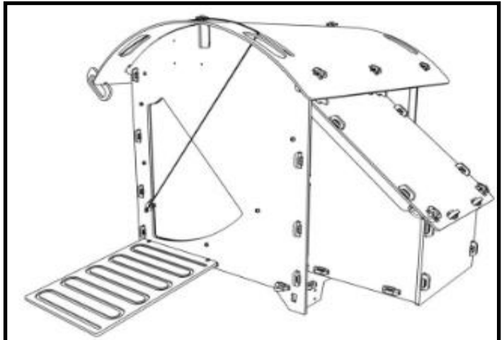
20 MANUAL DOOR ONLY: Tie one end of the Cord to the Split Ring in the Front Door and the other to the small hole in the Door Handle. The Cord should pass through the handle slot. Adjust the length of the cord so that, when the door is fully raised, the handle just hooks onto the edge of the opposite handhold or the roof edge
