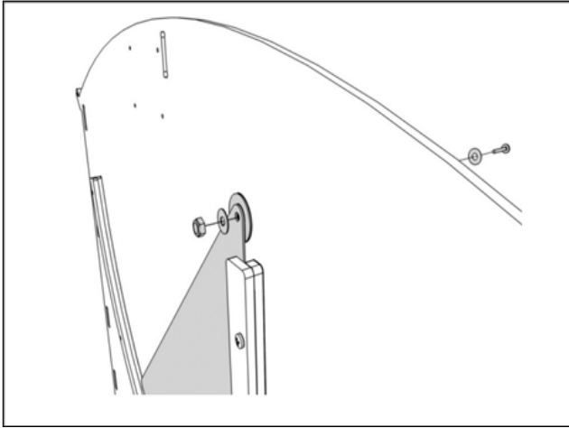
5 , Place the Metal Door in position, and secure it with a 20mm screw, 2x Standard Washers, a 25mm Washer and 1 x Nylock Nut. Tighten the Nylock Nut until the door can just rotate freely.
