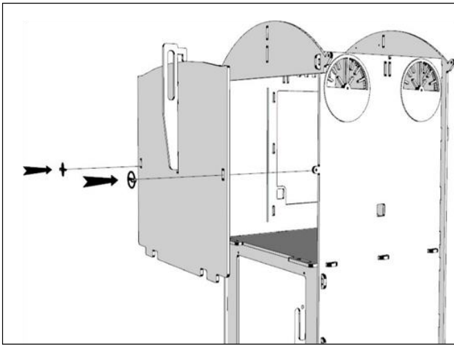
11, Fit the Back Door using 2x Lynch Pins. (When fitting, first rest the bottom of the Back Door in the slots in the Base, then push the door onto the lugs, and slide the Back Door Handles downwards. Secure it with Lynch Pins.
