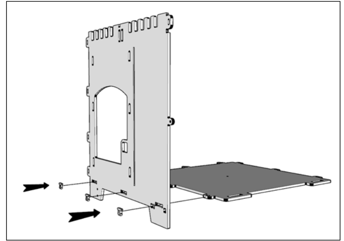
6 , Fit the nest box Side Wall to the Base using 3 x Pi Clips. Ensure that the Double-hole lugs are at the front .
