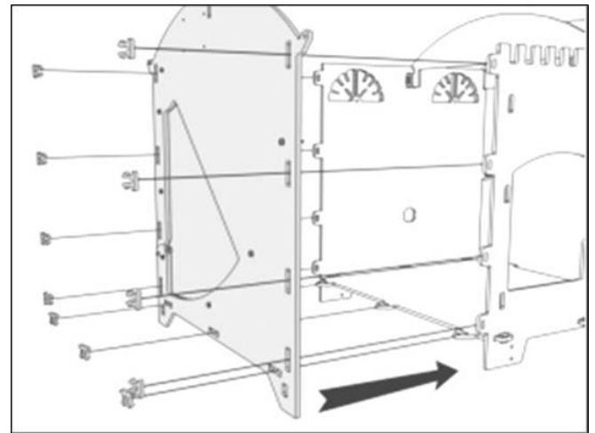
8 , Fit the Front Wall (patterned face outermost) to the end with the double-hole lugs using Pi Clips.
