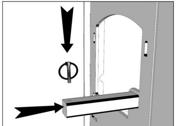
12, Slide the Perches through the Left and Right Side Walls and secure with a Lynch Pins at both ends.
