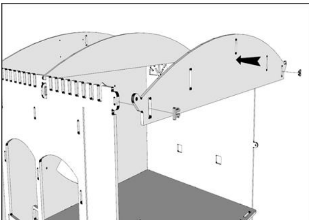
9 , Fit the Upper Back Wall to the top two lugs using 2 x Pi Clips. This is the same for large, medium and small.
