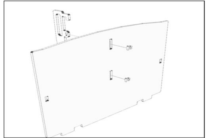
10 , Fit the Back Door Handle to the textured side of the back door using 2x Pi Clips. Hook on top of handle denotes the top.
