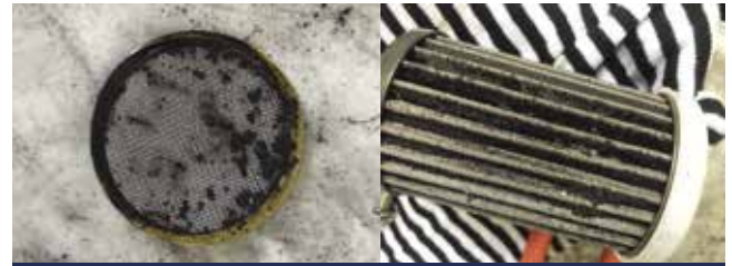
Reduced Flow Rate – Blocked Strainers in Bowser Pumps
