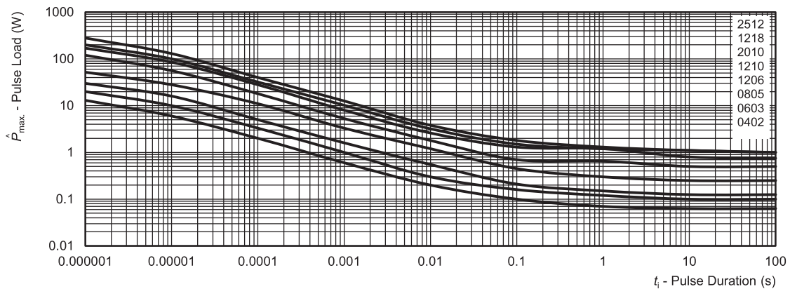
Maximum pulse load, continuous pulses; applicable if \bar{P} \leq P(\vartheta_{amb}) and \hat{U} = \hat{U}_{max} ; for permissible resistance change equivalent to 8000 h operation
