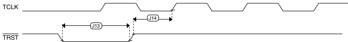
Figure 10. \overline{\text{TRST}} timing
