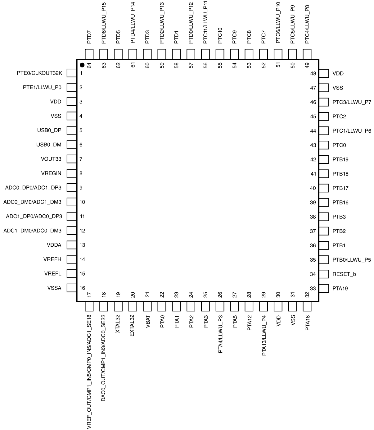
Figure 30. K22F 64 LQFP Pinout Diagram (top view)
