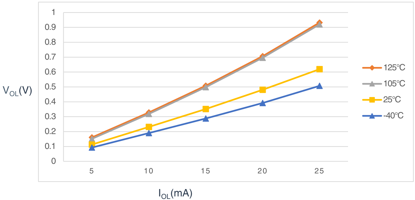
Figure 9. Typical I OL Vs. V OL (high drive strength) (V DD = 3 V)
