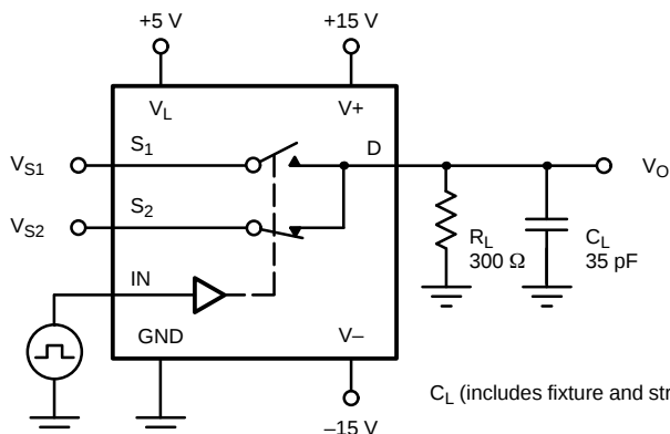
FIGURE 3. Break-Before-Make (DG419)
