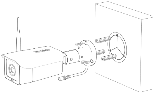
Wall Mount (Standard)
