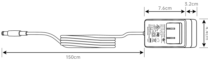
AC Power Adaptor (5.5x2.5mm Socket)
