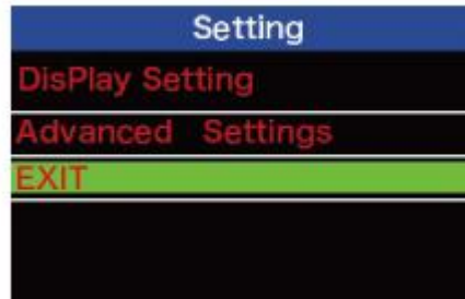
Setting interface
