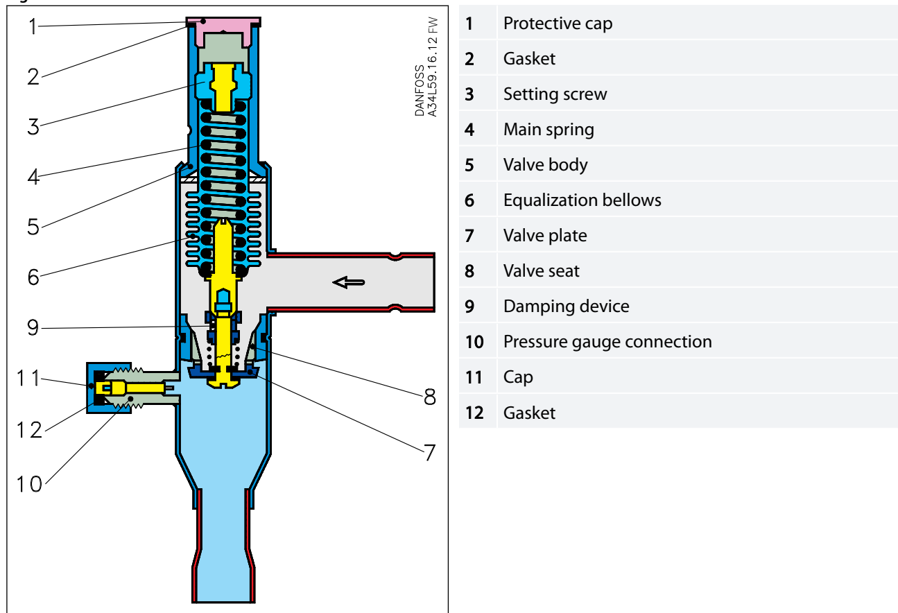
Figure 1: Function for KVD
