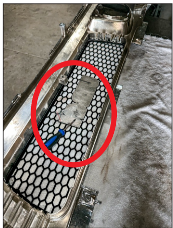
Flip grille over and place onto a towel so you do not scratch it and prepare the provided mounting hardware
