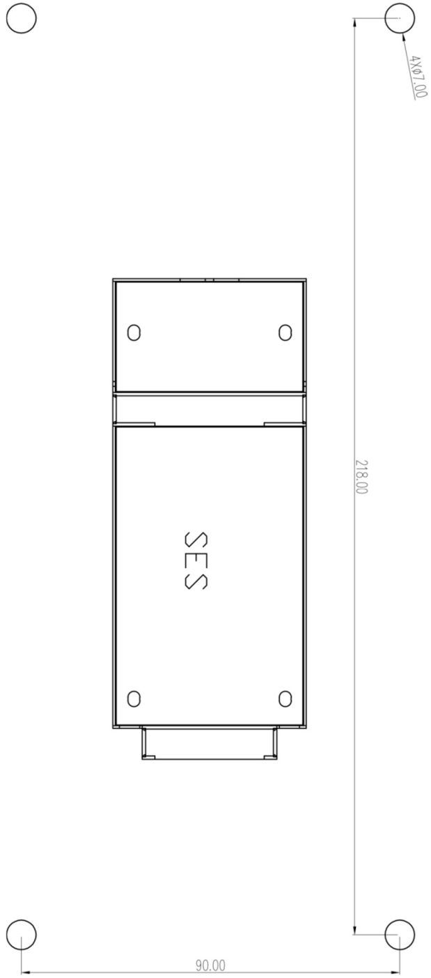
Installation drawing
