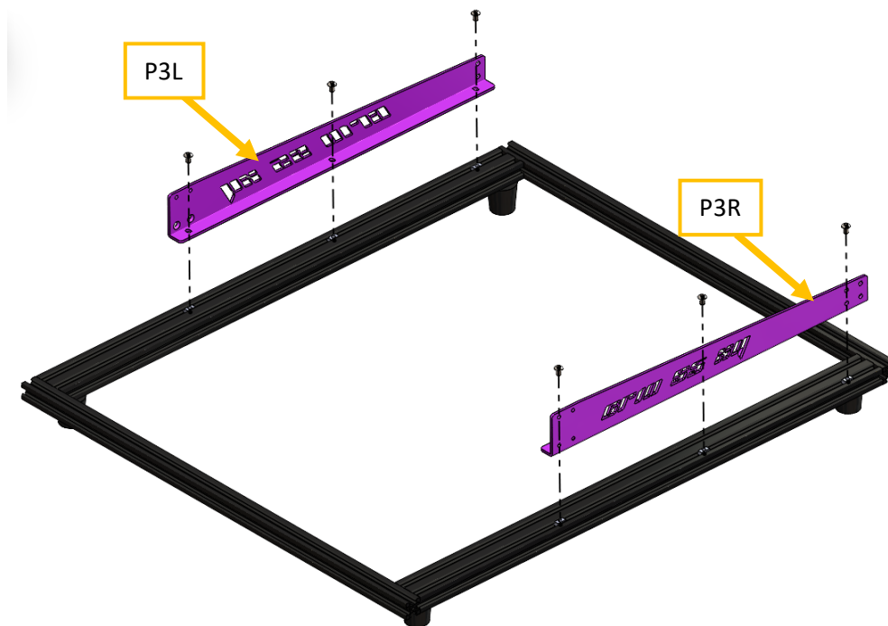
Figure 10 Bottom frame + P3 brackets.
