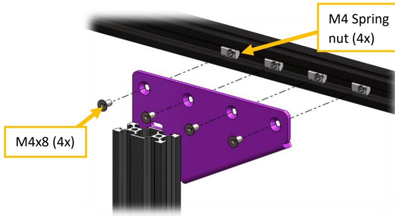
Figure 31 Front joint detail, M4x8 mm screws and nuts.
