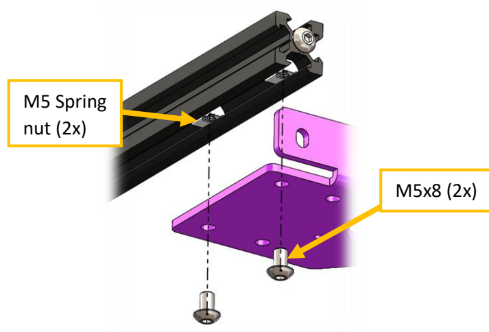
Figure 26 Fixing detail.
