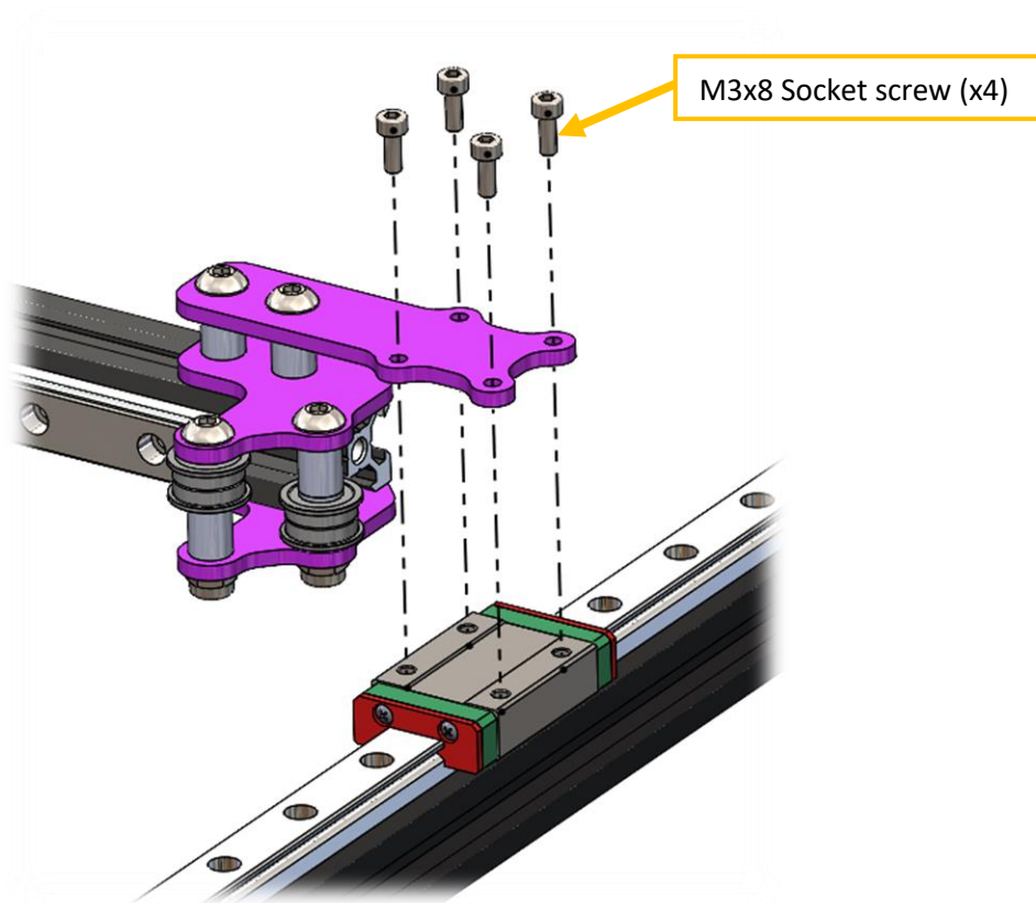
Figure 57 Right side X axis mount scheme.
