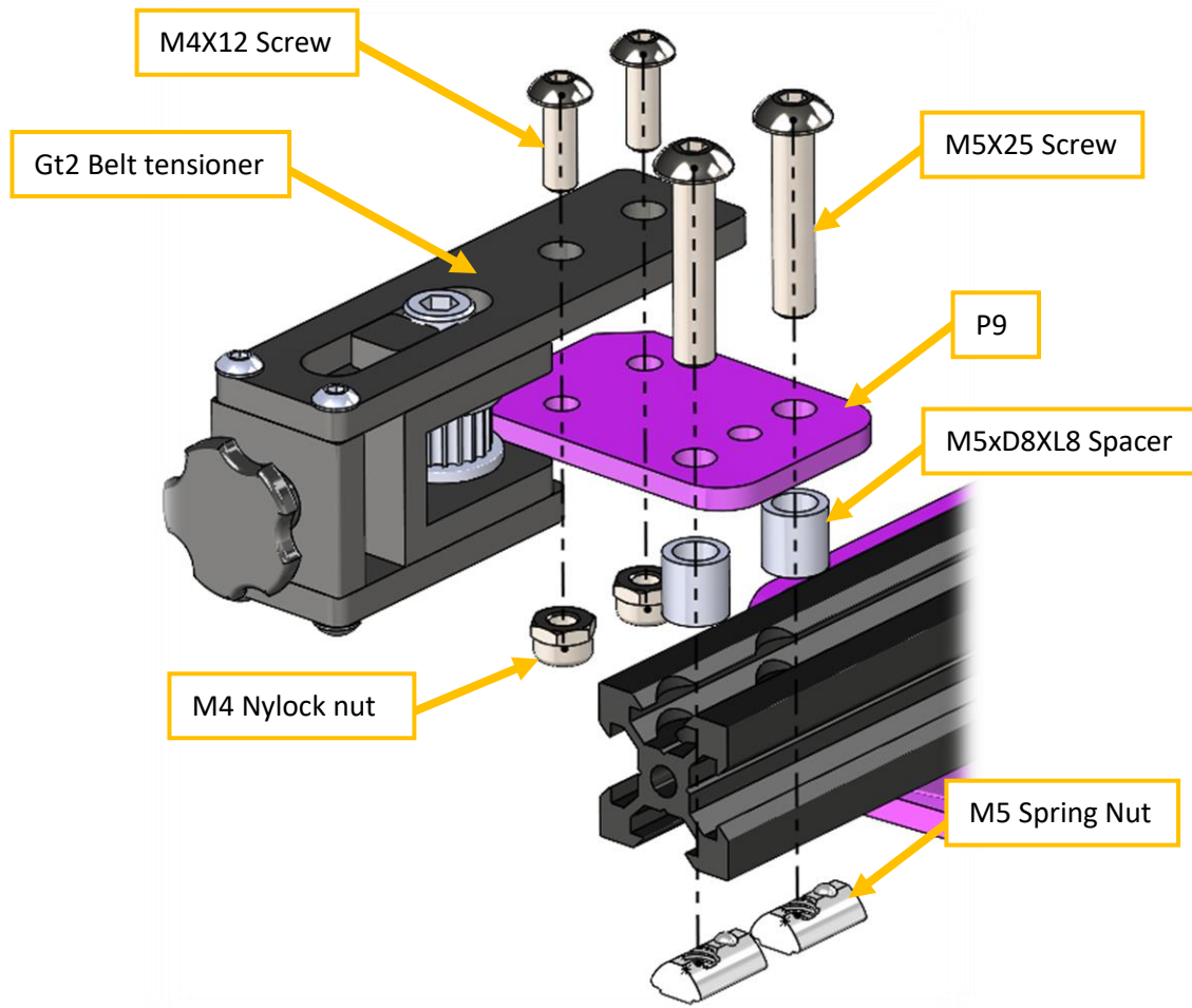
Figure 45 Right side belt tensioner mounting scheme.
