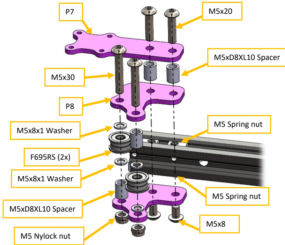
Figure 37 Left side X axis assembly scheme.
