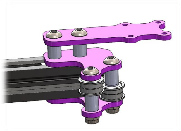
Figure 41 Right side mounted components.
