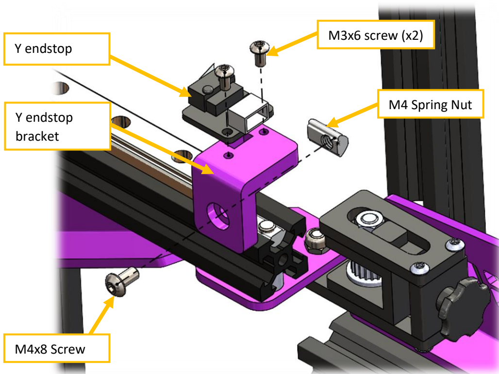
Figure 59 Y endstop mounting scheme.
