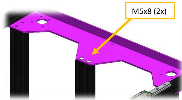
Figure 35 Detail of center extrusion fixing.
