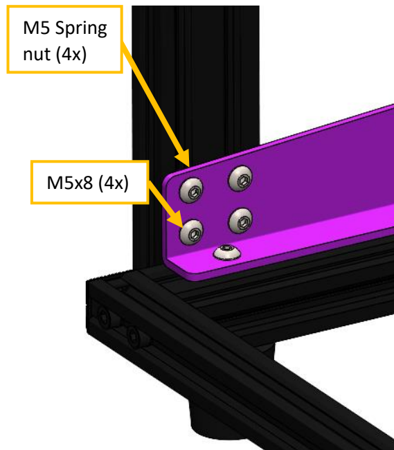
Figure 19 Detail of inner screws fixing.
