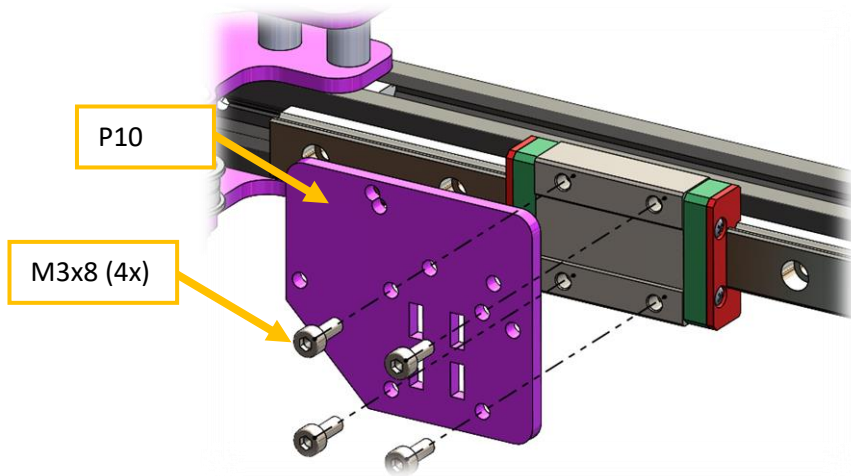
Figure 44 Hotend bracket mounting.
