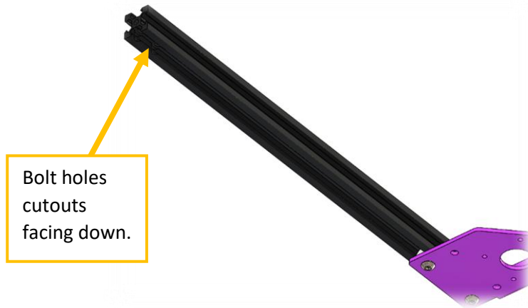
Figure 25 Left side 2020 extrusion detail.
