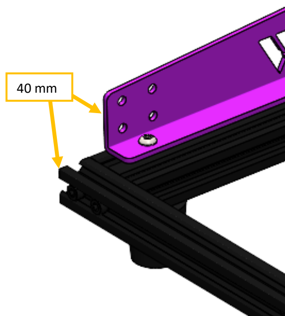
Figure 12 Keep 40mm between the edge of a frame and the bracket.
