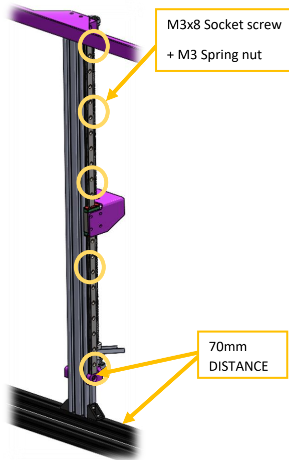
Figure 68 Z rails mounting, 3 rd rail is mounted at the left side of the 2040 extrusion.
