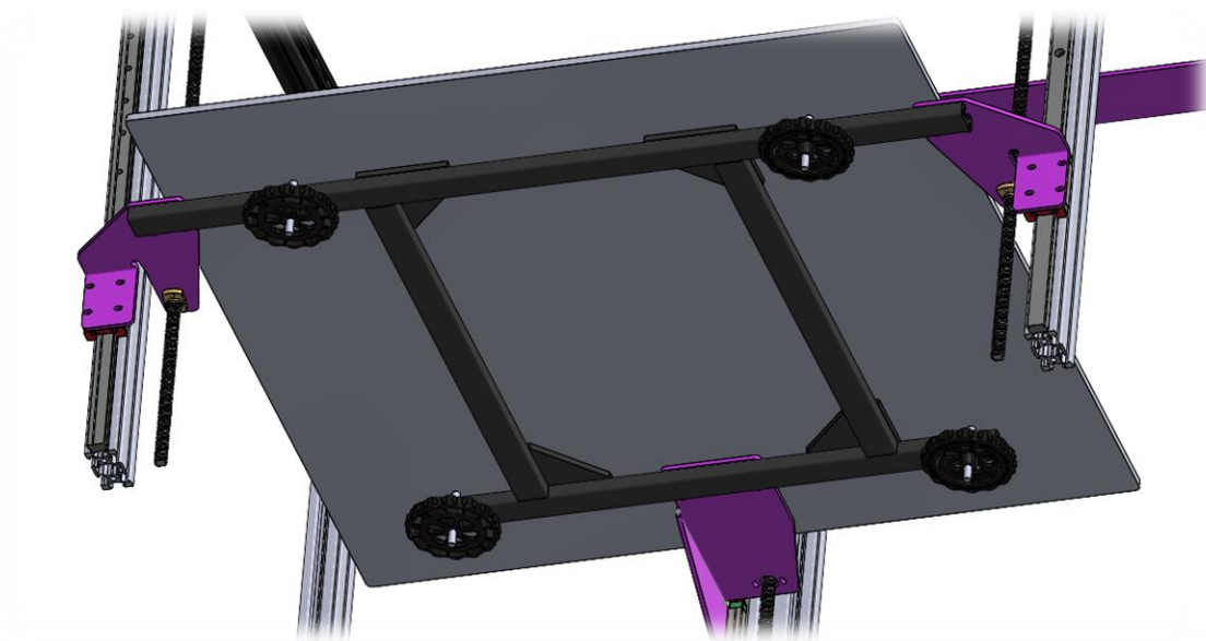
Figure 77 Bottom view for heatbed.
