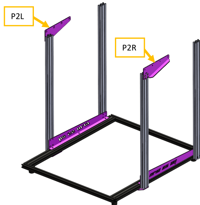
Figure 20 P2R/L bracket position.
