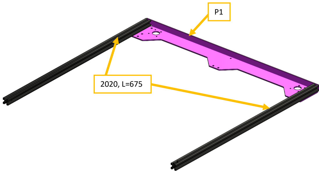
Figure 23 Top frame assembly.
