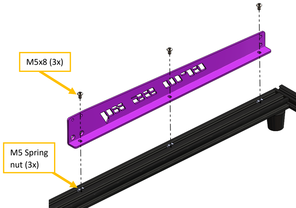
Figure 11 Joint detail with Screws and Spring nuts.
