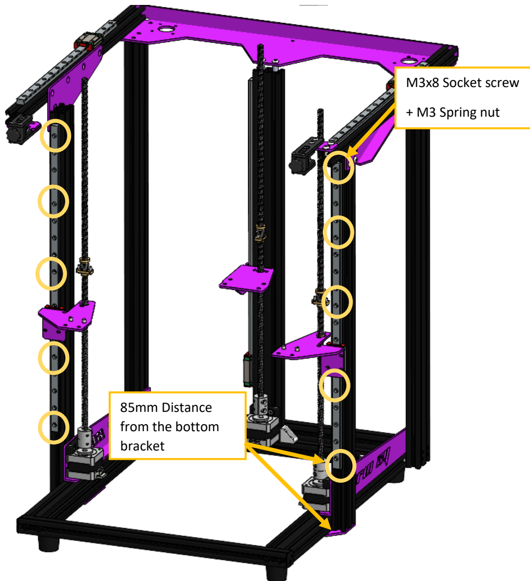
Figure 67 Z rails mounting.
