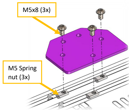
Figure 14 Fixing detail.
