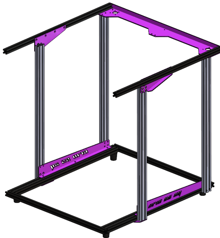
Figure 28 Frame assembly.
