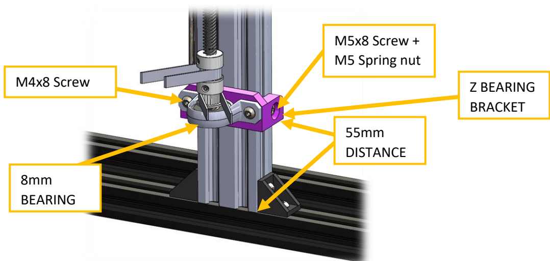
Figure 70 Z support mount detail (3 rd Z leadscrew)
