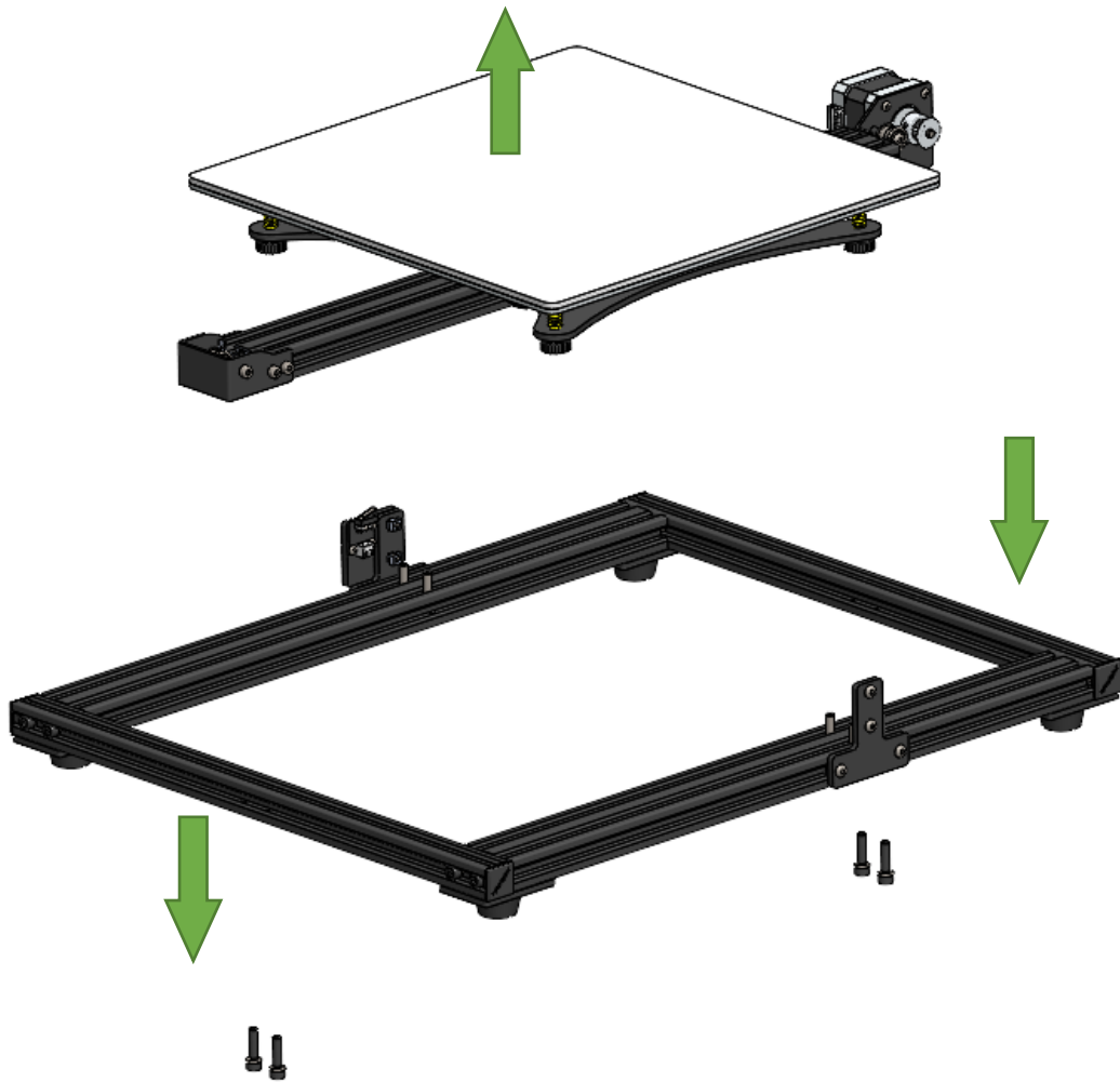
Figure 9 Removing Y axis and heatbed.
