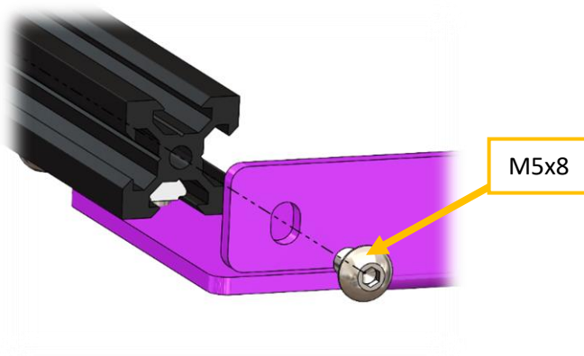
Figure 27 Back screw fixing detail.
