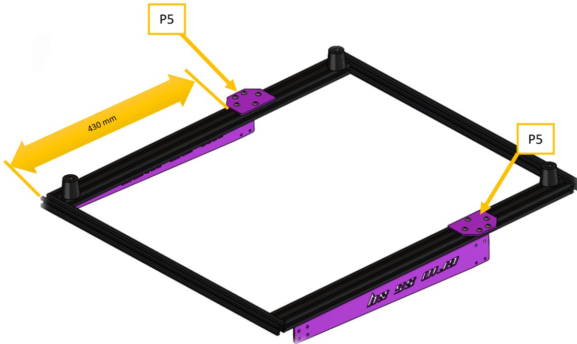
Figure 13 Bottom brackets mounting.
