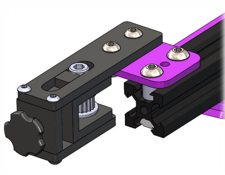
Figure 46 Right tensioner mount.
