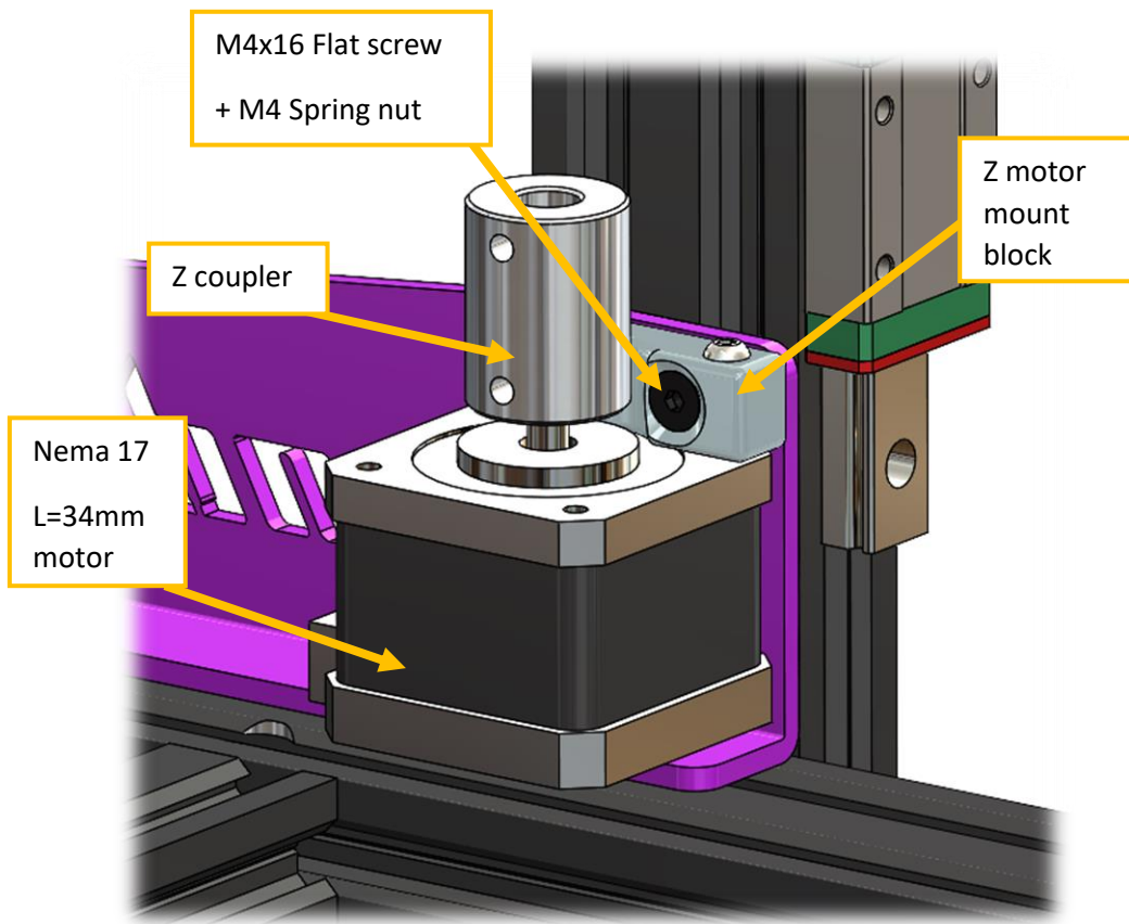
Figure 69 Z motor mount detail.
