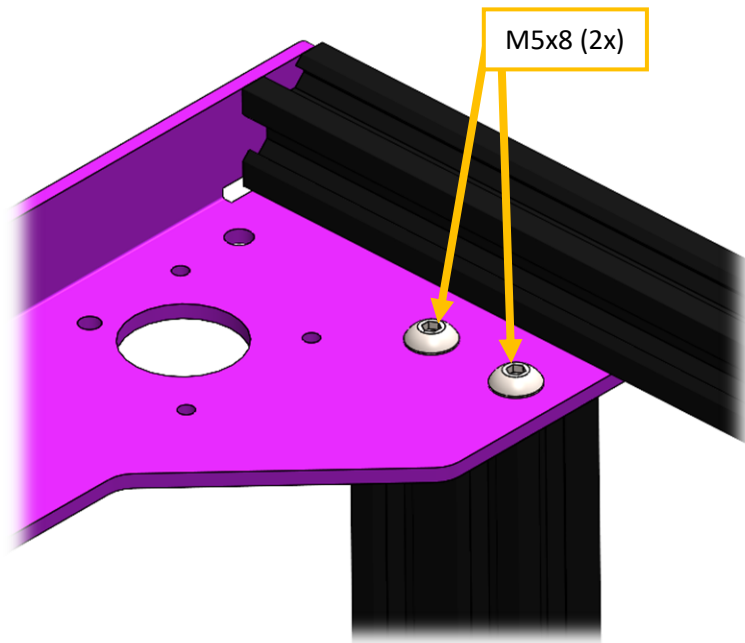
Figure 30 Back joint detail, M5x8 mm screw fixed to 2040 extrusion.
