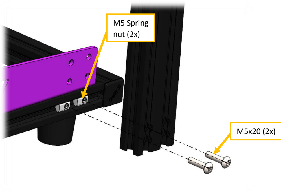
Figure 18 Detail of extrusion mounting.
