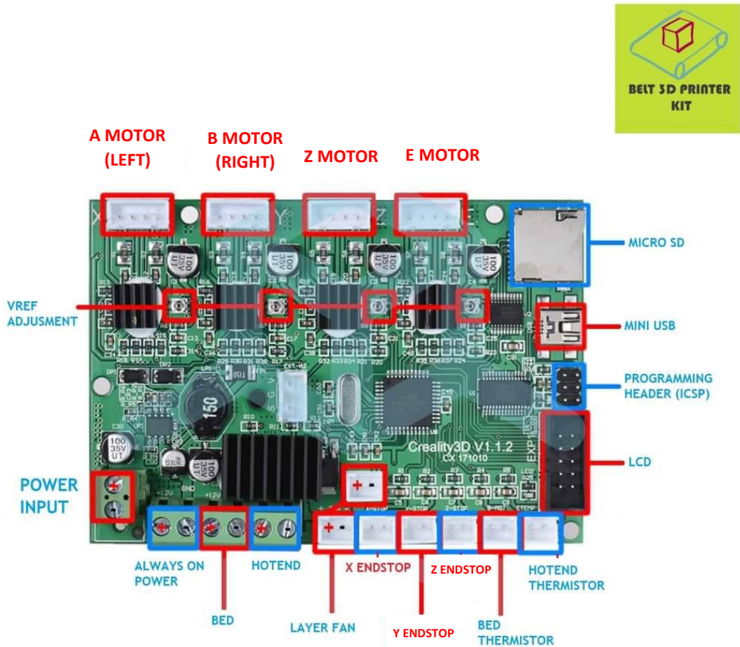
Figure 79 Wiring scheme for each component.
