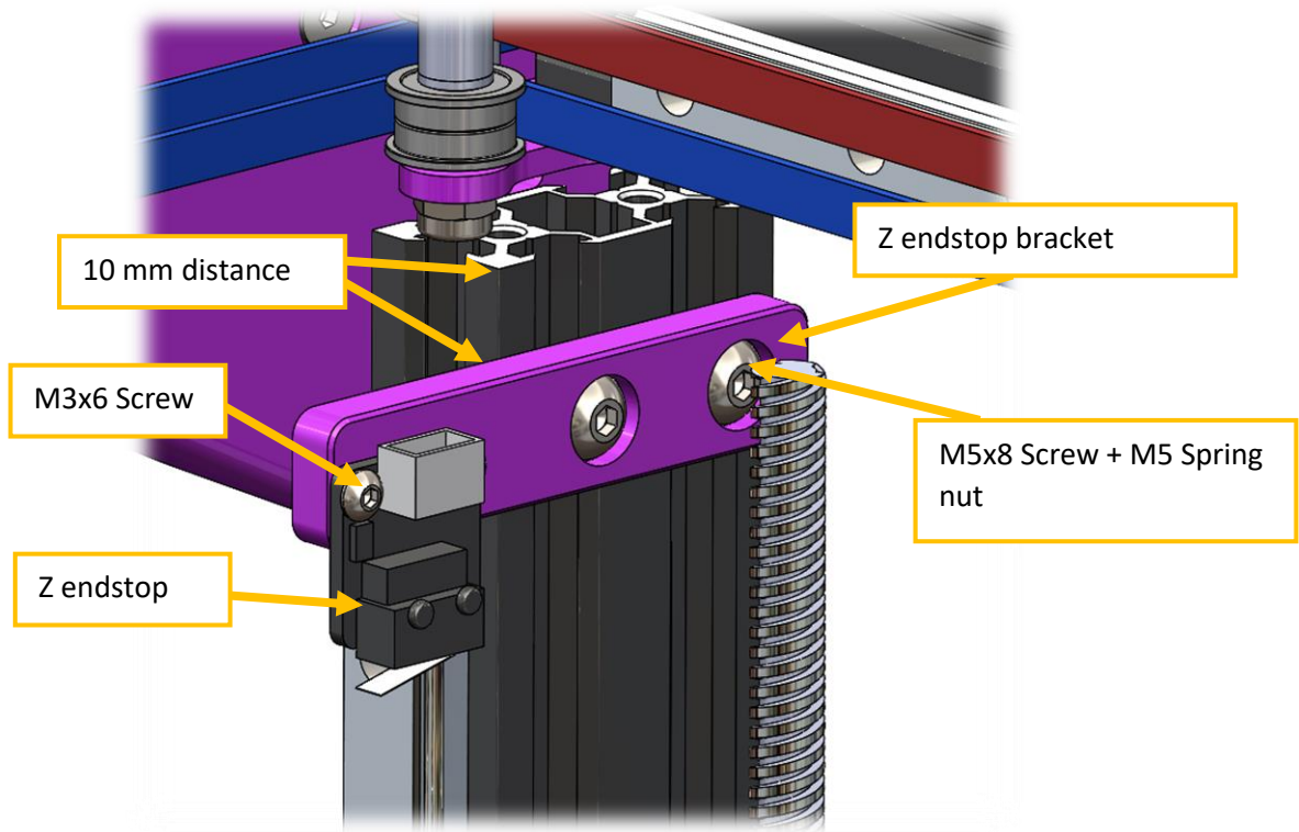
Figure 78 Z endstop bracket mounting.
