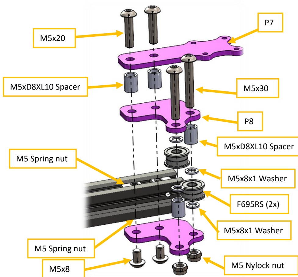
Figure 40 Right side X axis assembly scheme.
