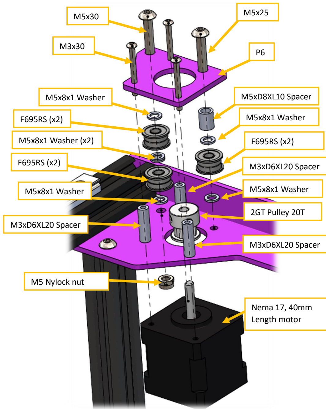
Figure 51 Left side Nema + Pulleys mount scheme.
