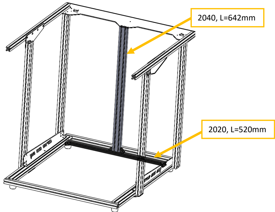
Figure 34 Detail of middle extrusions fixing.
