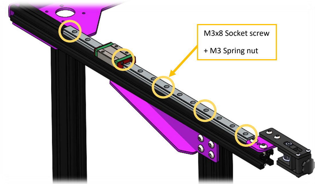
Figure 50 Left side, fix rails with M3x8 Screws + M3 Spring nuts were indicated with circles.
