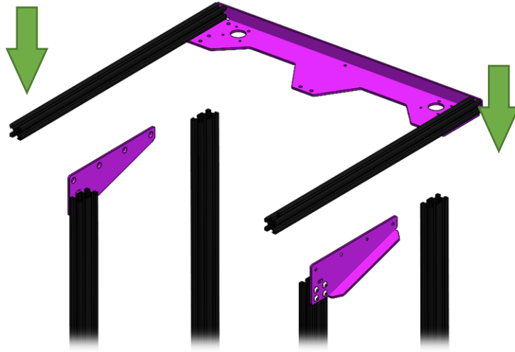
Figure 29 Assembly of top and bottom frames.
