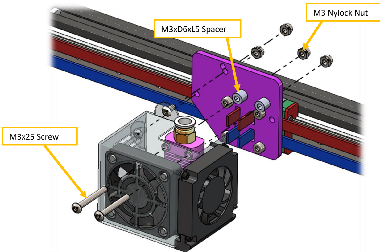
Figure 64 Stock Hotend Cr-10/PRO mounting scheme.
