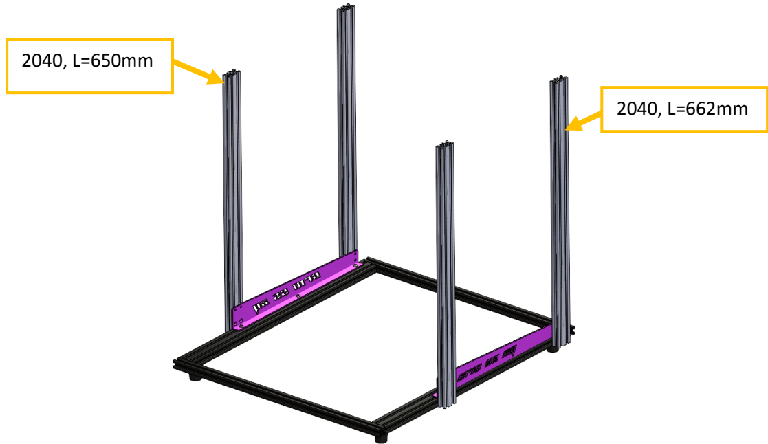
Figure 15 Installing 2040 Alu extrusions to the bottom frame.
