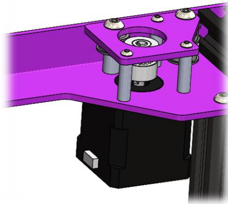
Figure 54 Right side motor mount finished.
