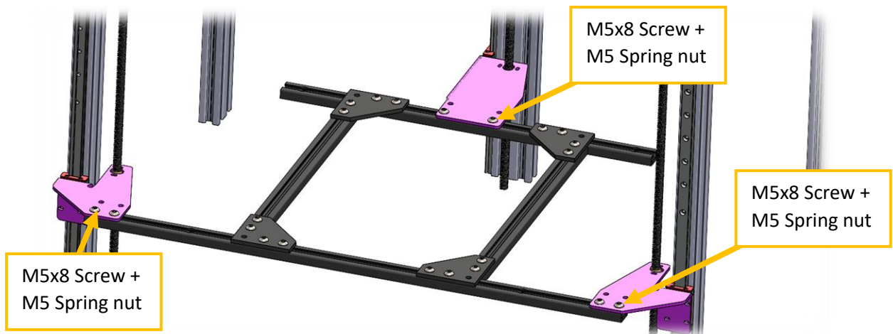
Figure 76 Top view for the bed bracket assembly.
