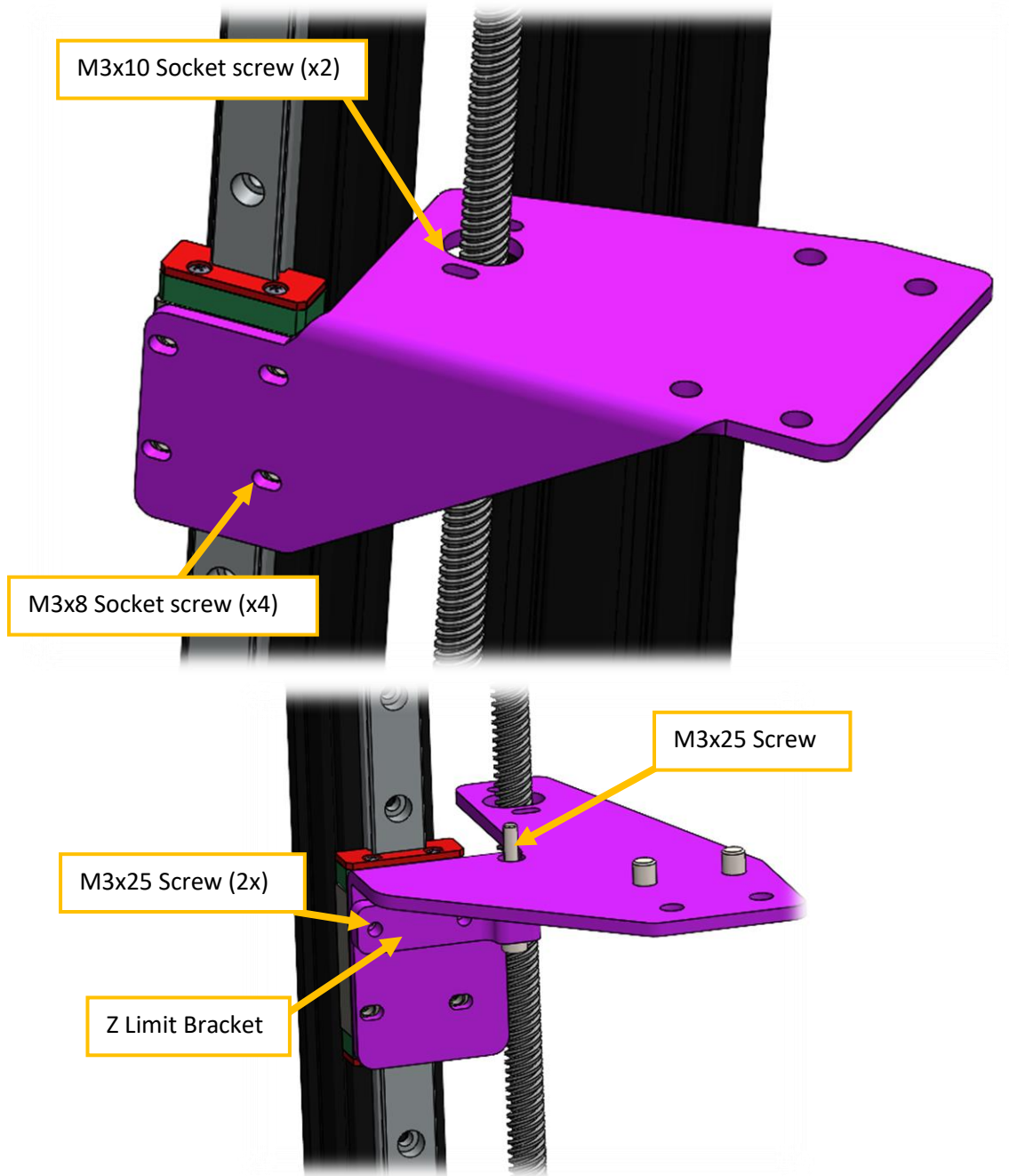
Figure 75 Left side detail.
