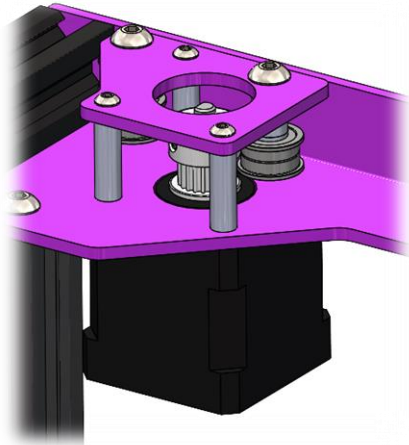
Figure 52 Left side motor mount finished.
