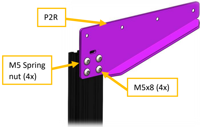
Figure 21 mounting detail for P2R bracket.
