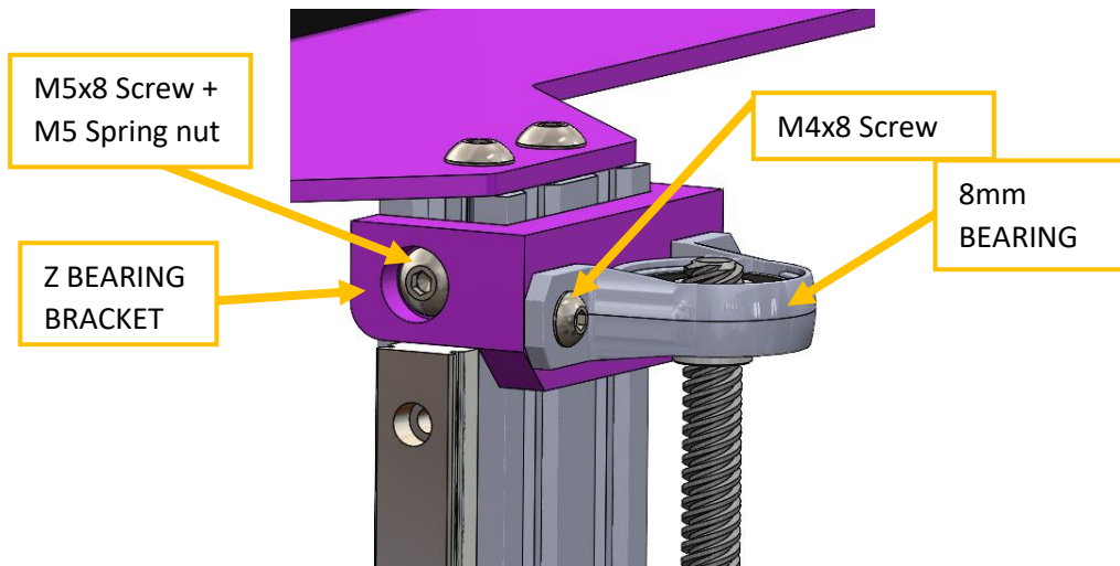
Figure 72 Top Bearing support detail, bracket is installed upside down.
