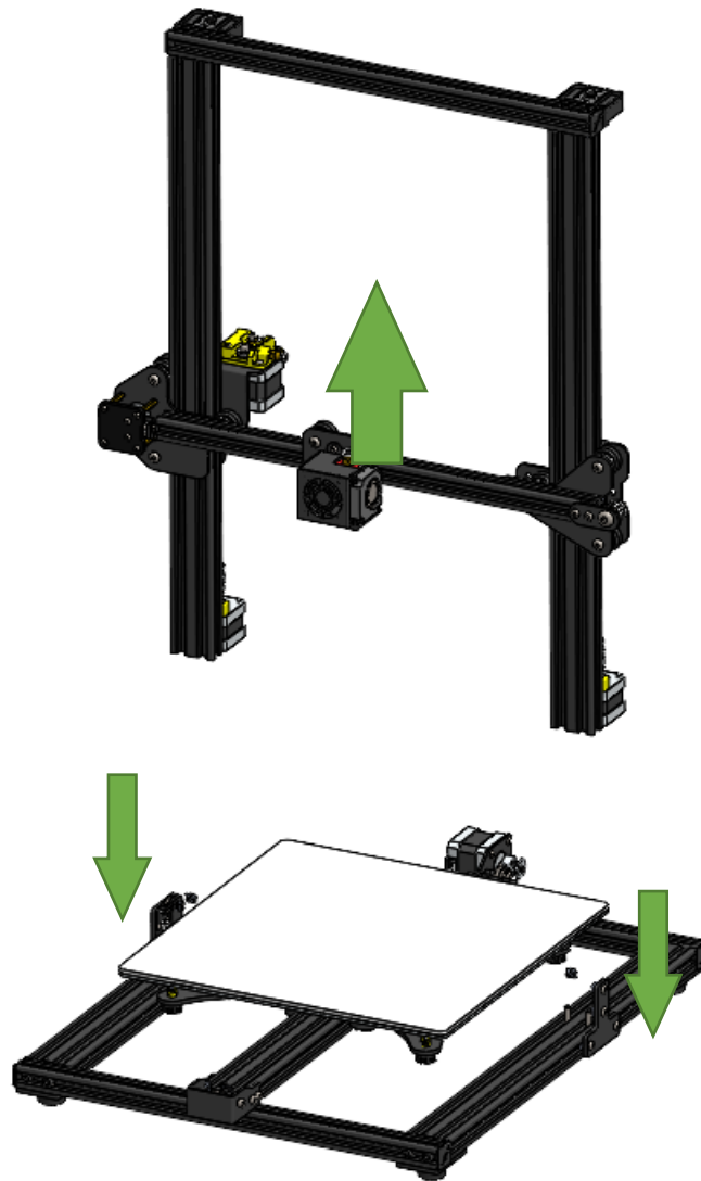
Figure 8 Removing top frame and X axis system.
