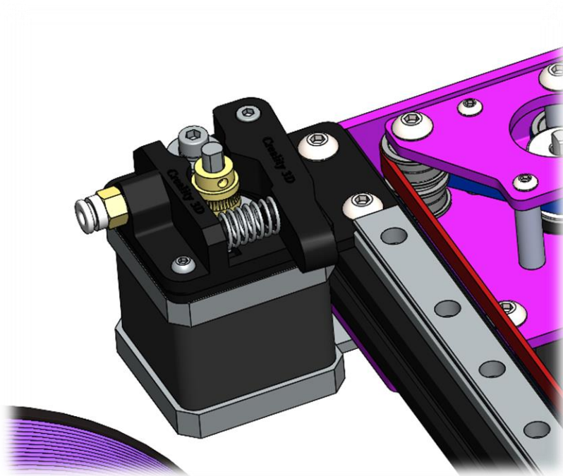
Figure 65 Suggested extruder position.
