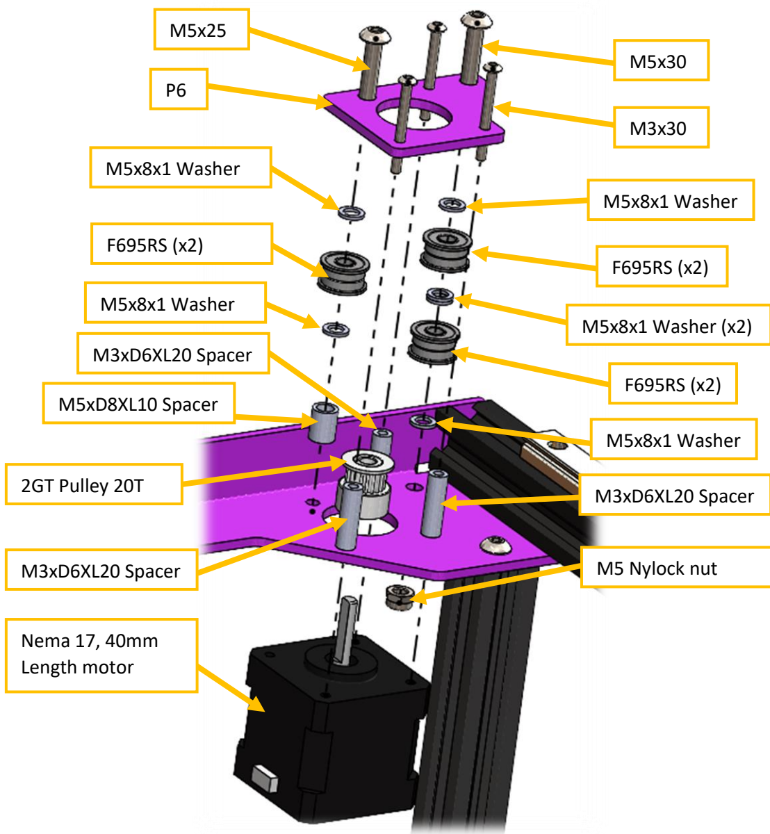
Figure 53 Right side Nema + Pulleys mount scheme.
