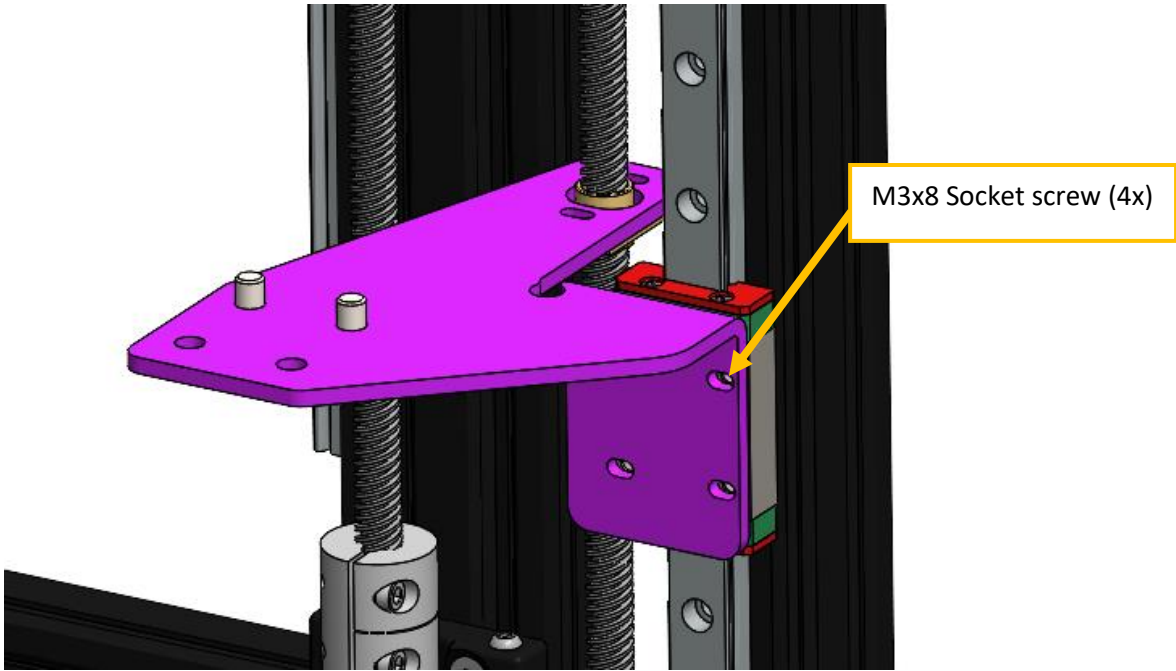
Figure 74 Right side detail.
