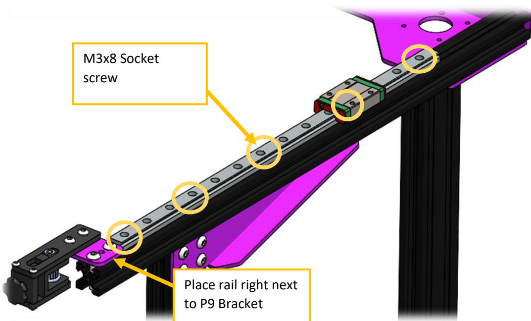
Figure 49 Right side, fix rail with M3x8 Screws + M3 Spring nuts were indicated with circles.
