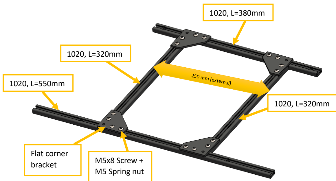
Figure 66 Heatbed base plate.
