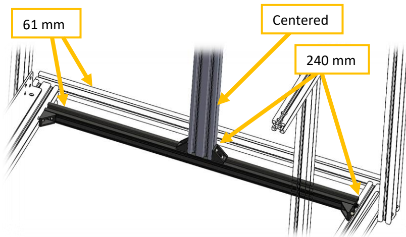
Figure 34 Detail of middle extrusions fixing.
