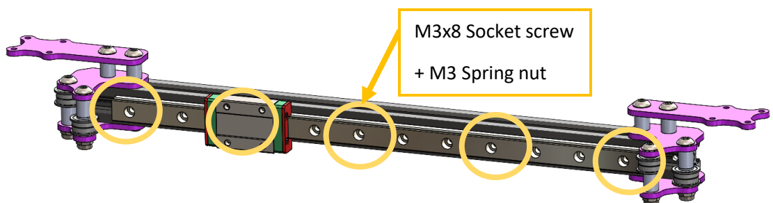
Figure 43 Fix rails with M3x8 Screws + M3 Spring nuts were indicated with circles.
