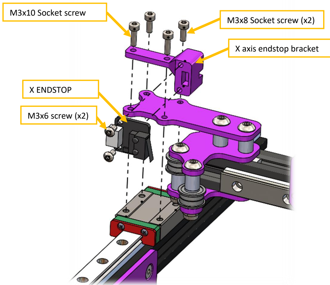
Figure 55 Left side X axis mount scheme.
