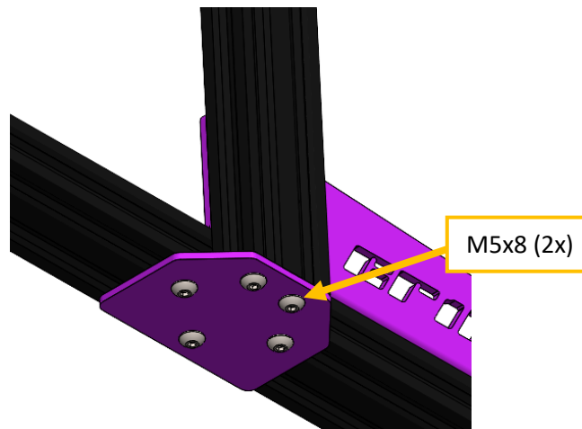
Figure 16 Mounting detail.
