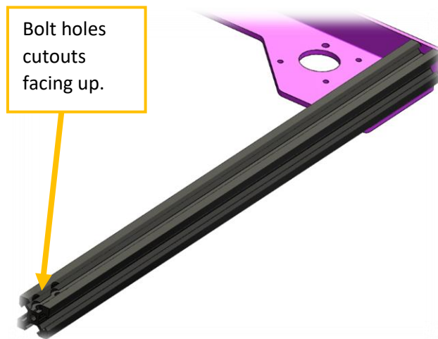
Figure 24 Right side detail for the 2020 extrusion.
