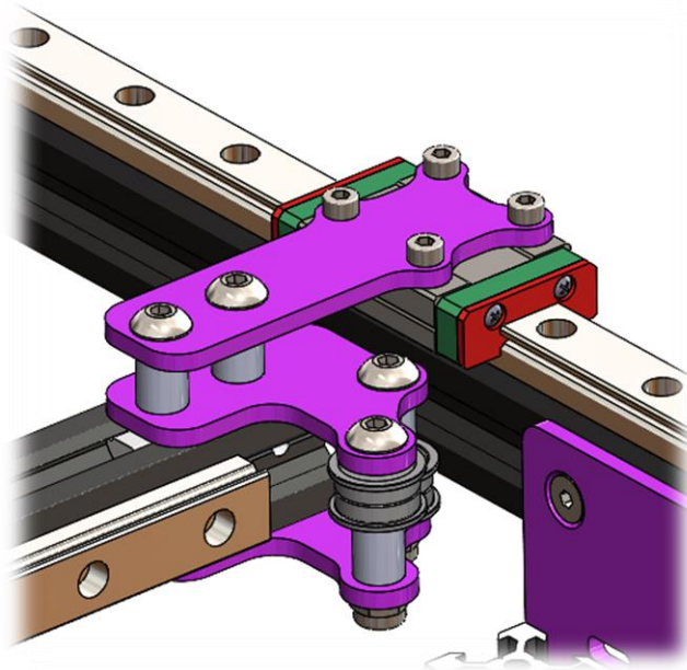
Figure 58 Right side detail of X mounting.
