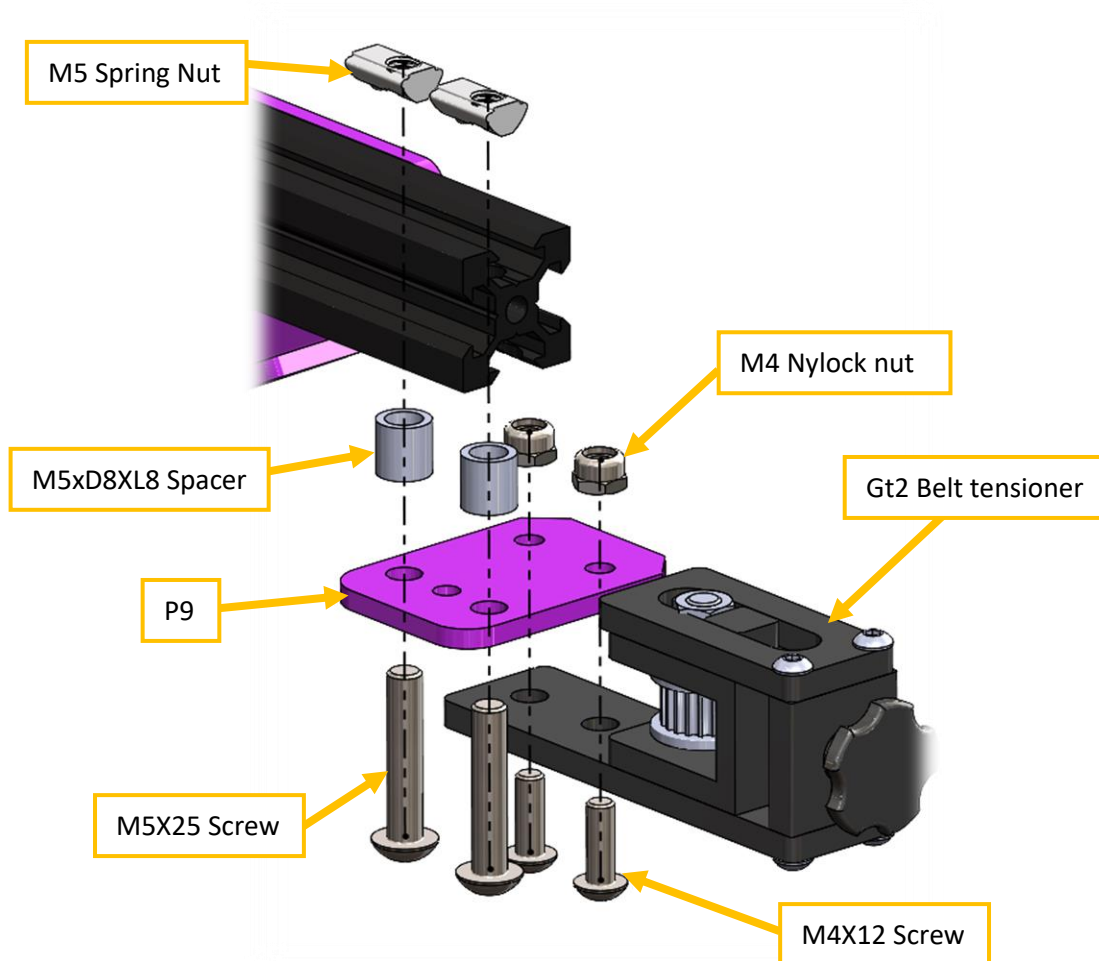
Figure 47 Left side belt tensioner mounting scheme.
