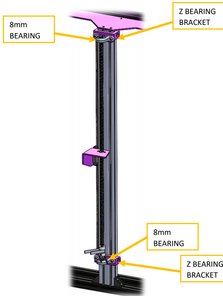
Figure 70 Z support mount detail (3 rd Z leadscrew)
