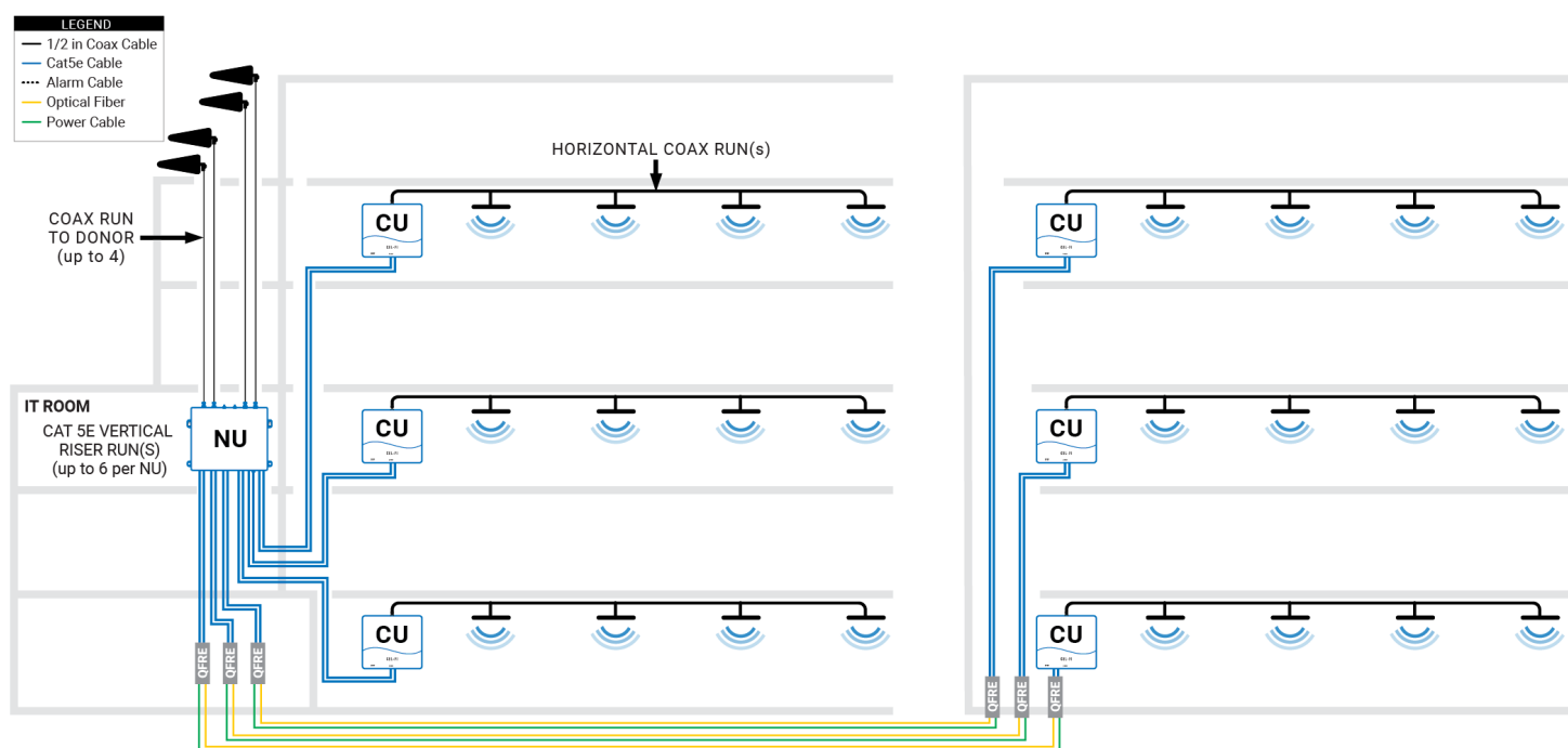
TWO-BUILDING DIAGRAM: 1 NU to 6 CUs with QUATRA Fiber Range Extenders
