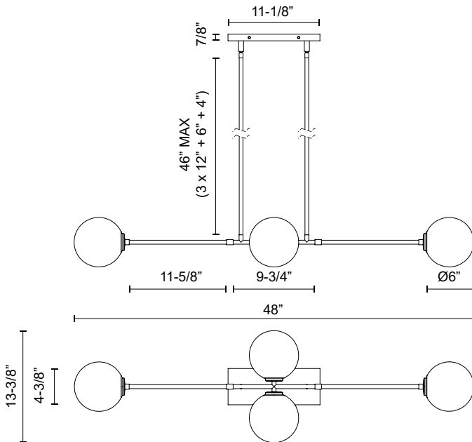
LP549448MBOP Matte Black/Opal Matte Glass
