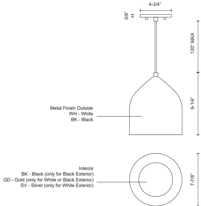
49108-WH/SV White/Silver
