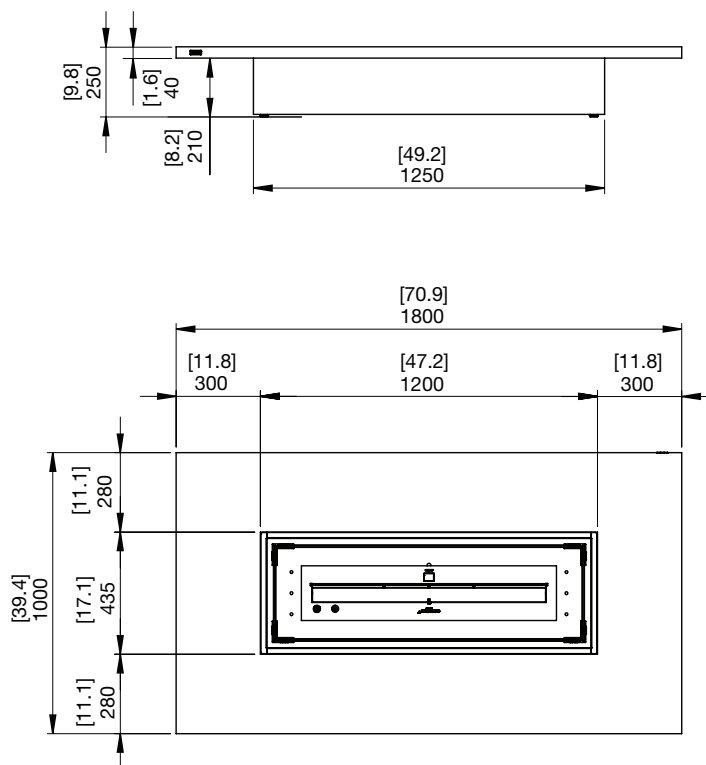
Line drawings show concrete models without a Fire Screen. Refer to the Fire Screen model specifications for dimensions.
