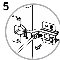
Front screws adjustment
