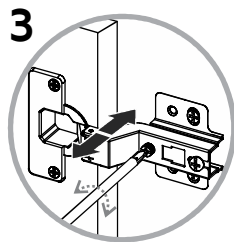
Lateral adjustment
