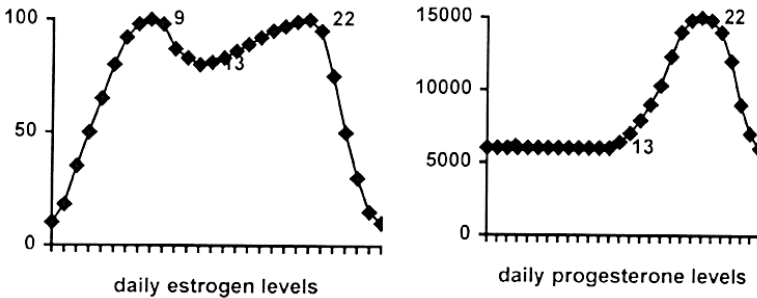
Fig. 21 Estrogen and progesterone levels (pg./ml)
