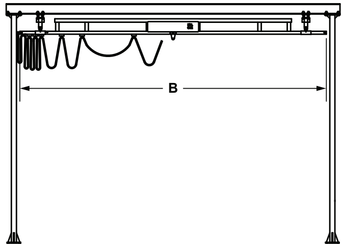
END VIEW
