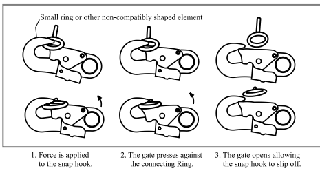
Figure 4 - Unintentional Disengagement (roll-out)
