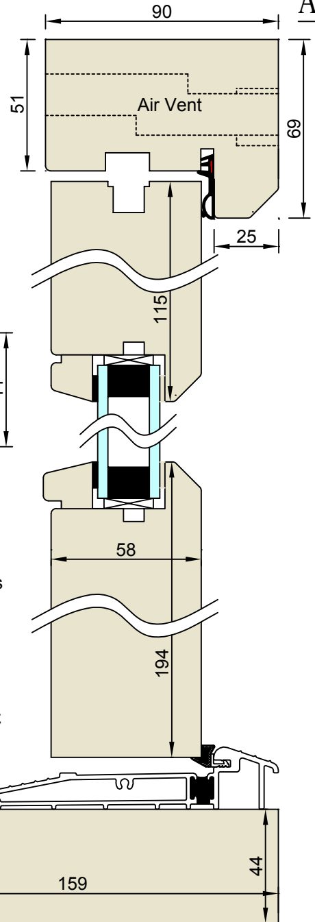
Head Detail Section A-A
