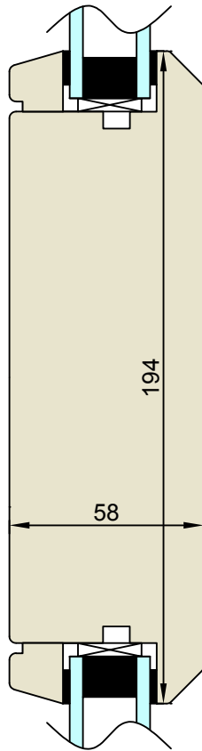
Transom Detail Section B-B
