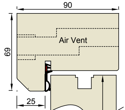
Head Detail Section A-A
