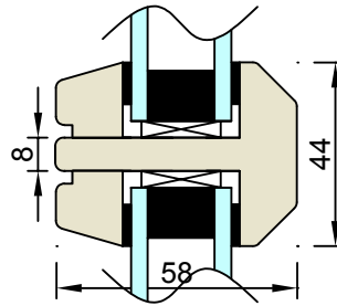
Standard 44mm Glazing Bar/Optional Plant-On Bars
