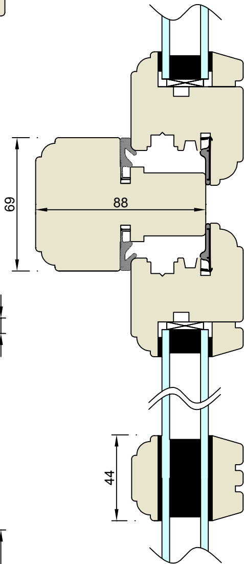
Transom Detail Section B-B
