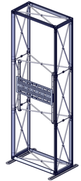
COMPLETE SETUP
