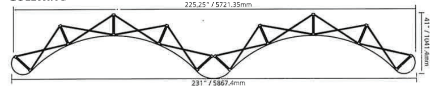
GULLWING
