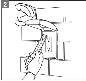
2 Measure outlet face. (Exposed outlet only.)
