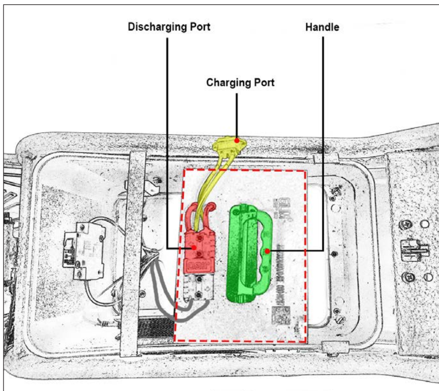
Removable Lithium Battery
