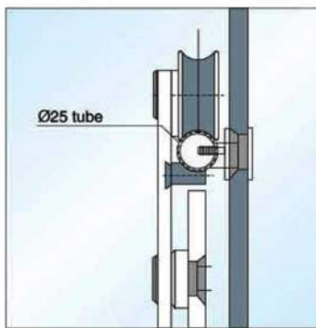
26602-044 CLAMP FIXING FOR WALL
