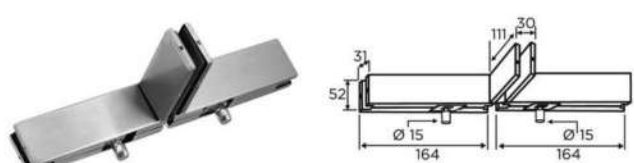
OVER PANEL CONNECTOR FOR BACK TO BACK DOORS
