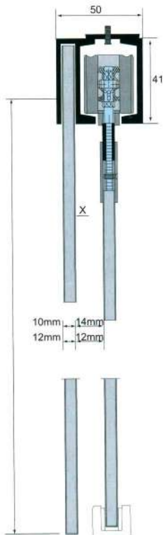
OVERHEAD TRACK WITH 1 MOVABLE PANEL & 1 FIXED PANEL
