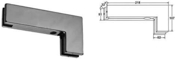
26201-C OVER PANEL SIDE PANEL CONNECTING PATCH WITH STRIKE INSERT
