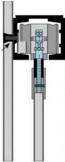
15026-GC GLASS TO TRACK CLAMP
