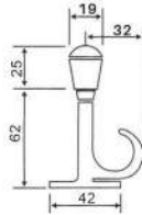
35118 WALL MOUNT
