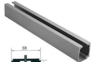
15026-T (1 Pc.) OVERHEAD CHANNEL 120"
