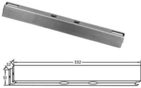
26201-DR OVER PANEL DOUBLE DOOR STRIKE
