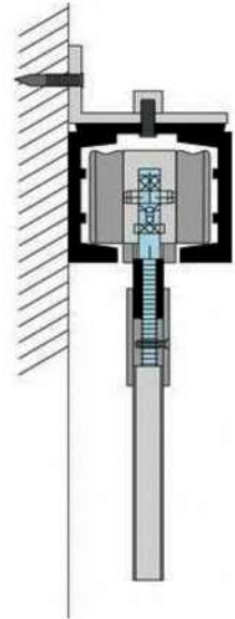
SIDE WALL MOUNTED DOOR ASSEMBLY
