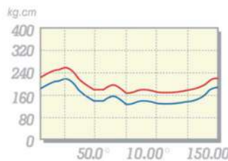
Shown curves refer to PDC103W
