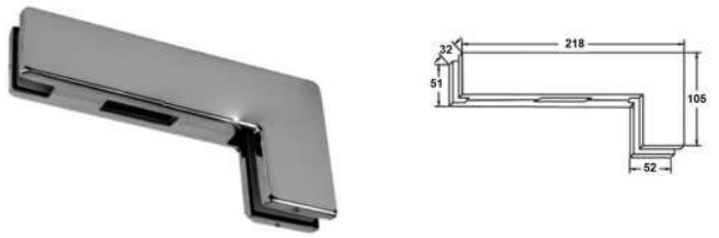
26201-B OVER PANEL SIDE PANEL CONNECTING PATCH WITH STRIKE INSERT
