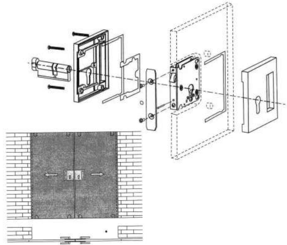
69006-01A GLASS TO GLASS DOOR LOCK
