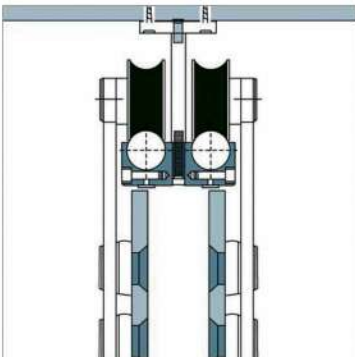
26602-020 DOUBLE TUBE TO CEILING CLAMP
