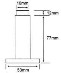
35112 WALL MOUNT
