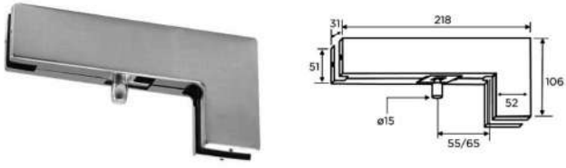
26201-A OVER PANEL SIDE PANEL CONNECTING PATCH WITH PIVOT
