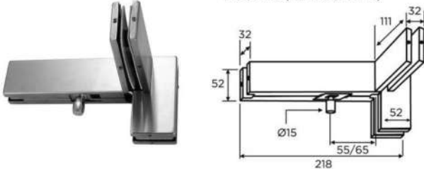
OVER PANEL SIDE PANEL CONNECTOR WITH FIN FITTING (RIGHT/LEFT)
