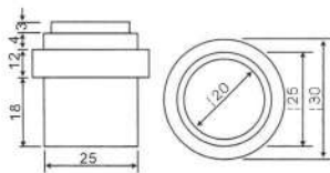
35120 FLOOR MOUNT
