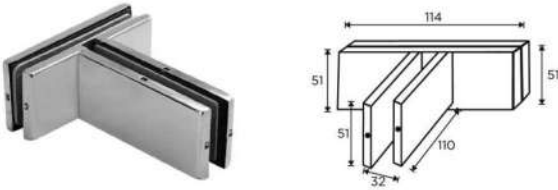
26230-WF DOUBLE GLASS CONNECTOR WITH FIN FITTING INSIDE
