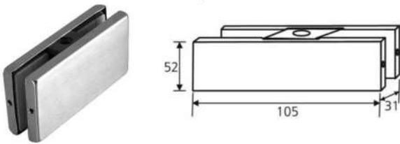
GLASS TO GLASS CONNECTING PATCH TO WALL/CEILING
