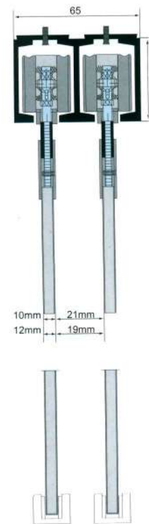
SIDE WALL MOUNTED DOOR ASSEMBLY
