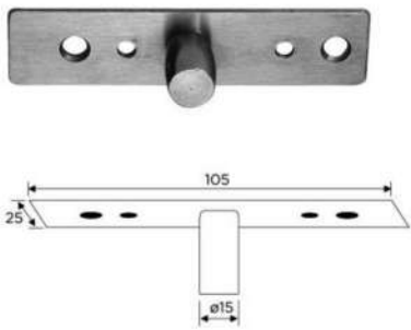
Pivot TOP PIVOT FOR PATCH / POINT FITTING DOORS
