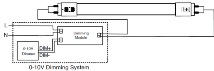
Direct AC wiring diagram with 0-10V dimming system
