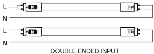
Direct AC wiring diagram
