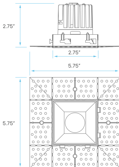
CUTOUT: 3.25" X 3.25"
