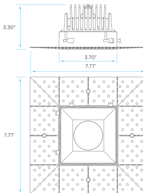
CUTOUT: 4.25" X 4.25" 4"
