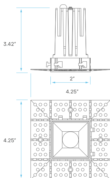
CUTOUT: 2.44" X 2.44"
