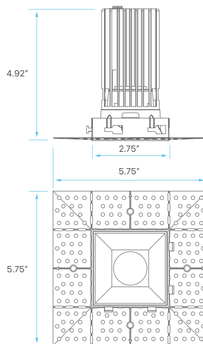
CUTOUT: 3.25" X 3.25"
