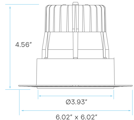
4" TRIMLESS CUTOUT: Ø 4.25"
