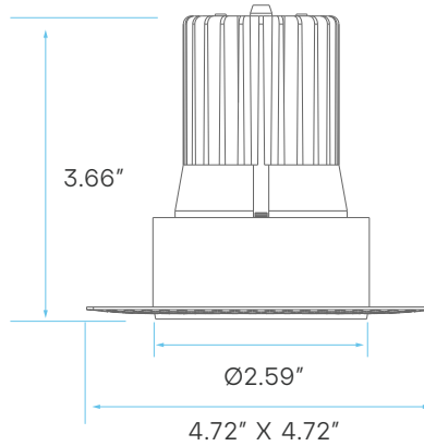
2" TRIMLESS CUTOUT: Ø 3"
