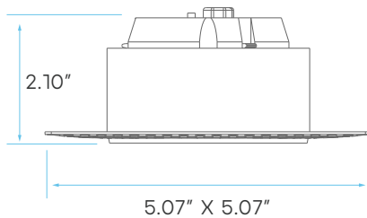
3" TRIMLESS - FLOATING GIMBAL CUTOUT: Ø 3.38"
