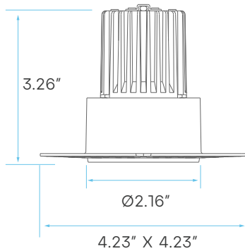
1" TRIMLESS CUTOUT: Ø 2.5"
