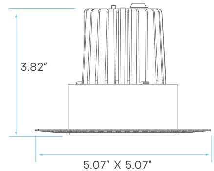
3" TRIMLESS - FLAT CUTOUT: Ø 3.38"
