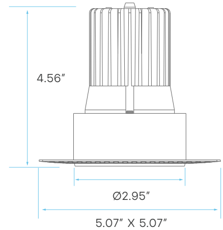
3" TRIMLESS CUTOUT: Ø 3.38"
