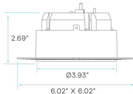
4" TRIMLESS - FLOATING GIMBAL CUTOUT: Ø 4.25"
