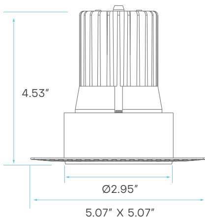
3" TRIMLESS - ZOOMABLE CUTOUT: Ø 3.38"
