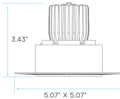
3" TRIMLESS - GIMBAL CUTOUT: Ø 3.38"
