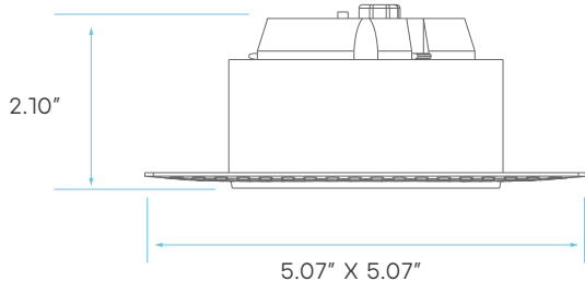
3" TRIMLESS - FLOATING GIMBAL CUTOUT: Ø 3.38"
