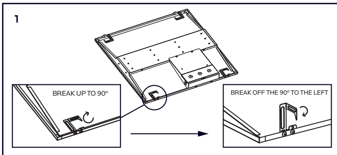
1. Remove the original ceiling tile for the Troffer.
