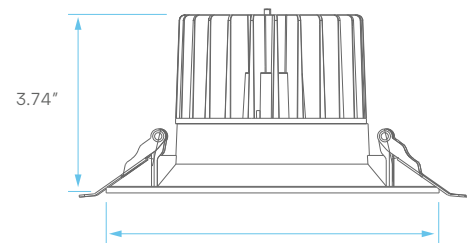
MODULE + 6" TRIM CUTOUT: Ø6.22"
