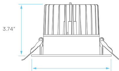
MODULE + 5" TRIM CUTOUT: Ø5.19"
