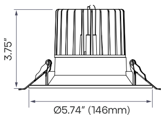
MODULE WITH 5" TRIM CUTOUT WITH 5" TRIM: Ø5.19" (132MM)
