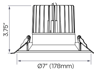
MODULE WITH 6" TRIM CUTOUT WITH 5" TRIM: Ø6.22" (158MM)
