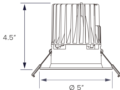
4" MODULE - CUTOUT: Ø 3.94" (100mm)
