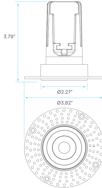
LR24917 CUTOUT: Ø 2.36"
