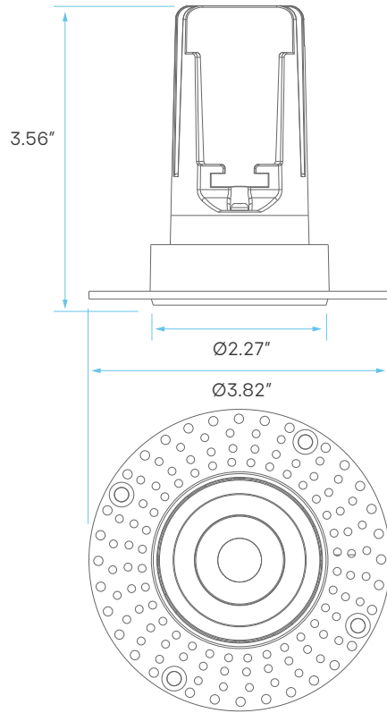
LR24916 CUTOUT: Ø 2.24"
