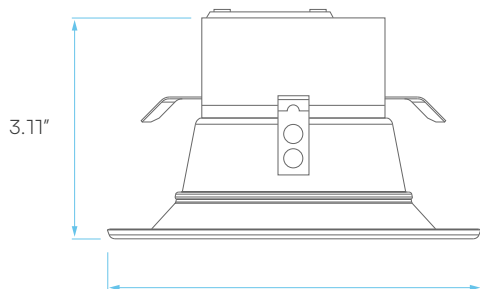
Ø5.09" ROUND
