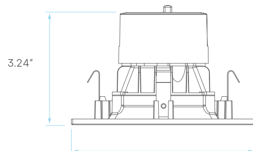
5" SQUARE
