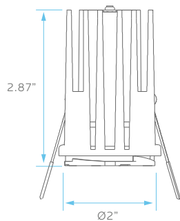
CUTOUT: Ø 2.12"
