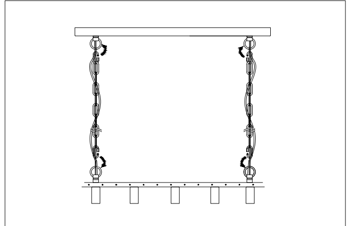
2. Determine the hanging length of the chandelier. Connect the chain according to the height needed. Thread the wires through the chains and ceiling canopy.
