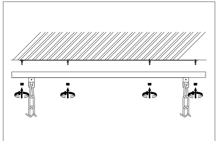
4. Place the canopy over the ceiling plate and fix it with the nuts.
